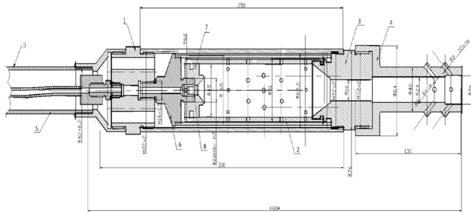
Figure 1-Thermal tool BVR80
