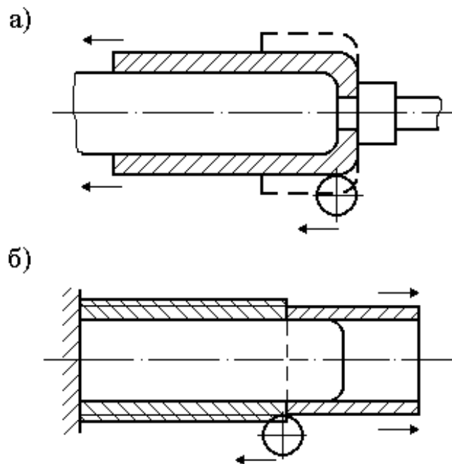
Figure 1 - Rotary drawing of a cylindrical thin-walled part by direct (a) and reverse (b) methods
