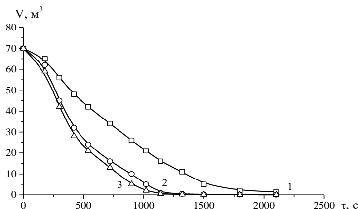
Figure 1 – Change in the estimated volume of oil mixtures from the Zhetybay, Uzen, Kalamkas, and Karazhanbas fields in a tank depending on the draining time.
